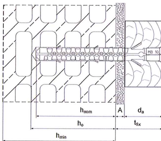
Installation in hollow brick (e.g. MB 10)
