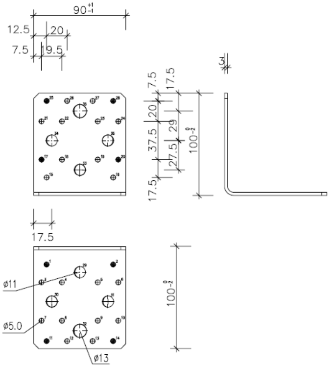
Figure A.6 Dimensions of Angle Bracket SXAB100
