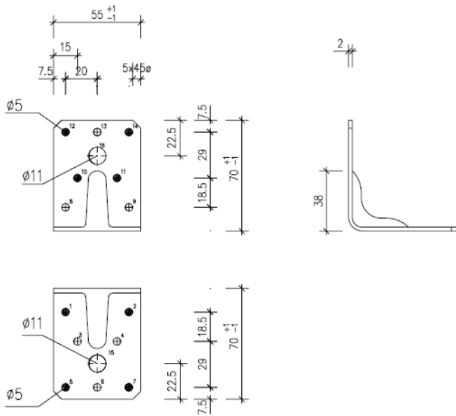
Figure A.1 Dimensions of Angle Bracket SXABR70
