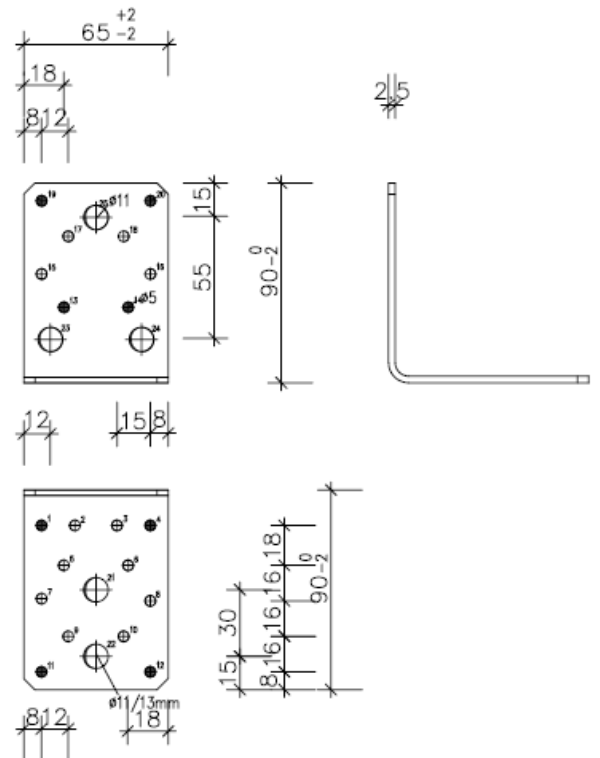
Figure A.4 Dimensions of Angle Bracket SXAB90, SXAB9013
