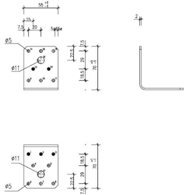
Figure A.2 Dimensions of Angle Bracket SXAB70
