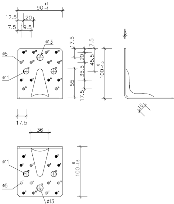
Figure A.5 Dimensions of Angle Bracket SXABR100
