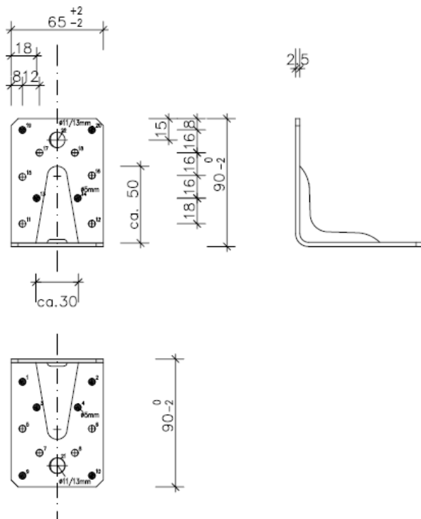
Figure A.3 Dimensions of Angle Bracket SXABR90, SXABR9013
